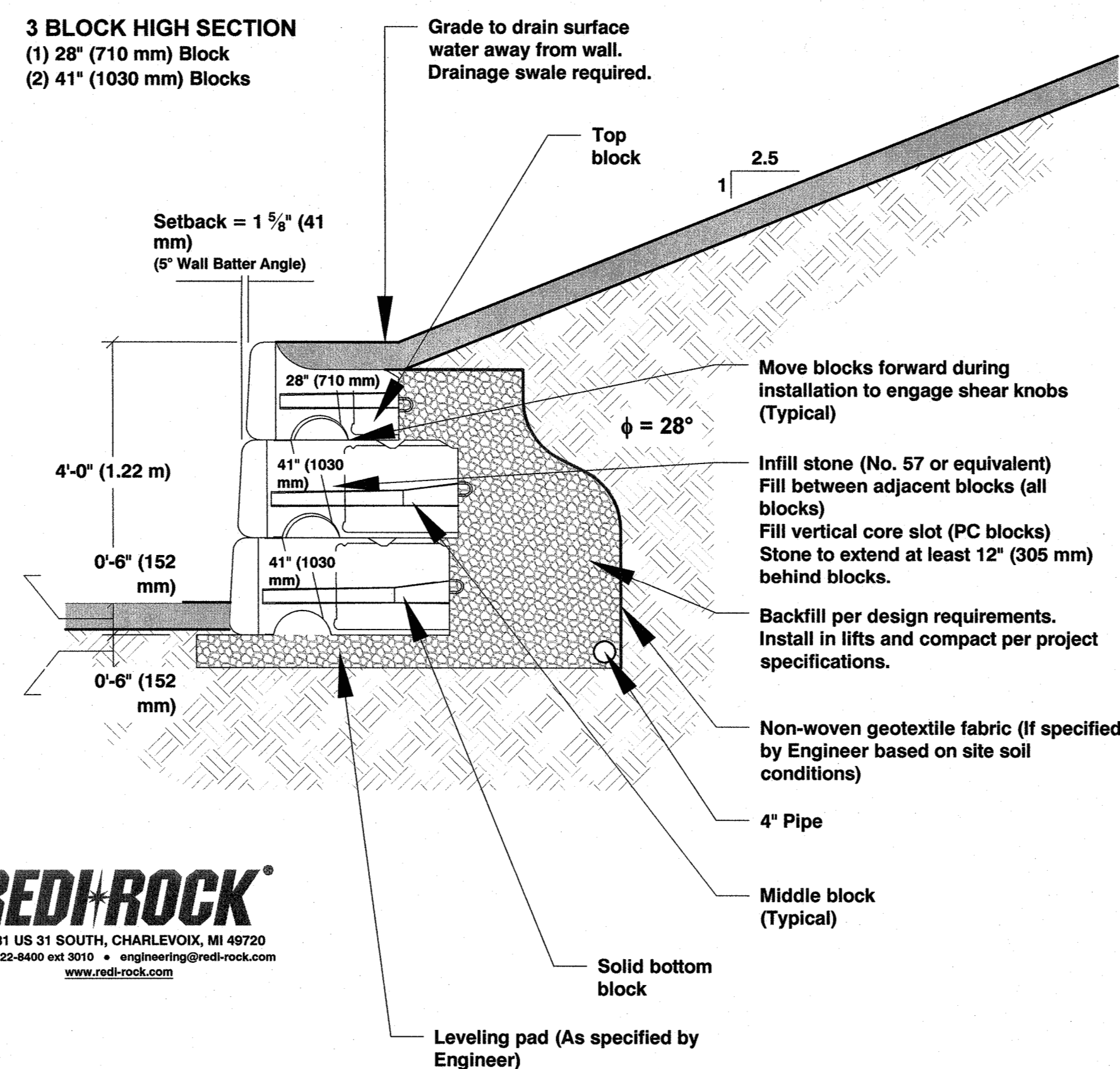
REDI ROCK WALL: 3 BLOCK SECTION
