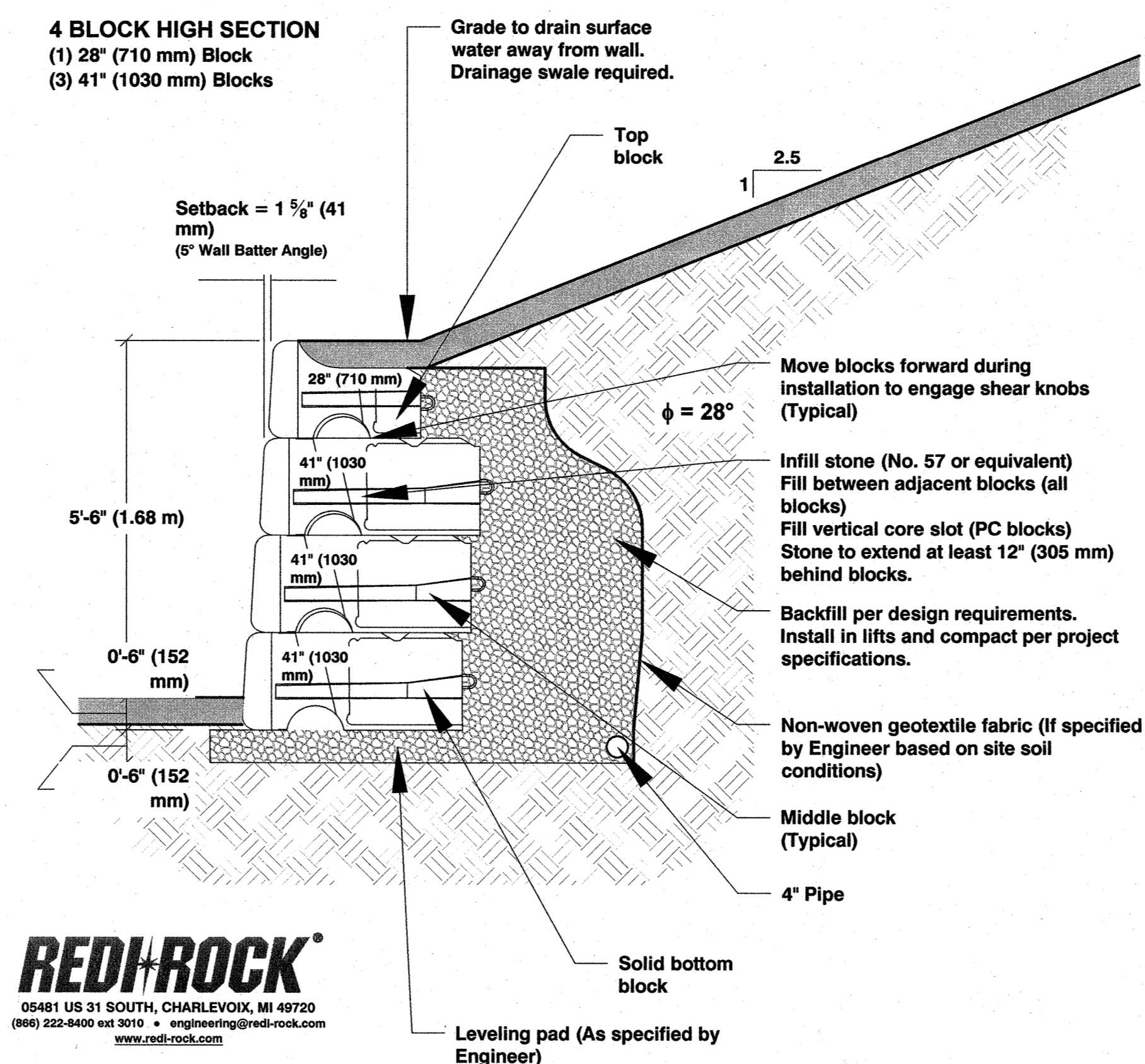
REDI ROCK WALL: 4 BLOCK SECTION
