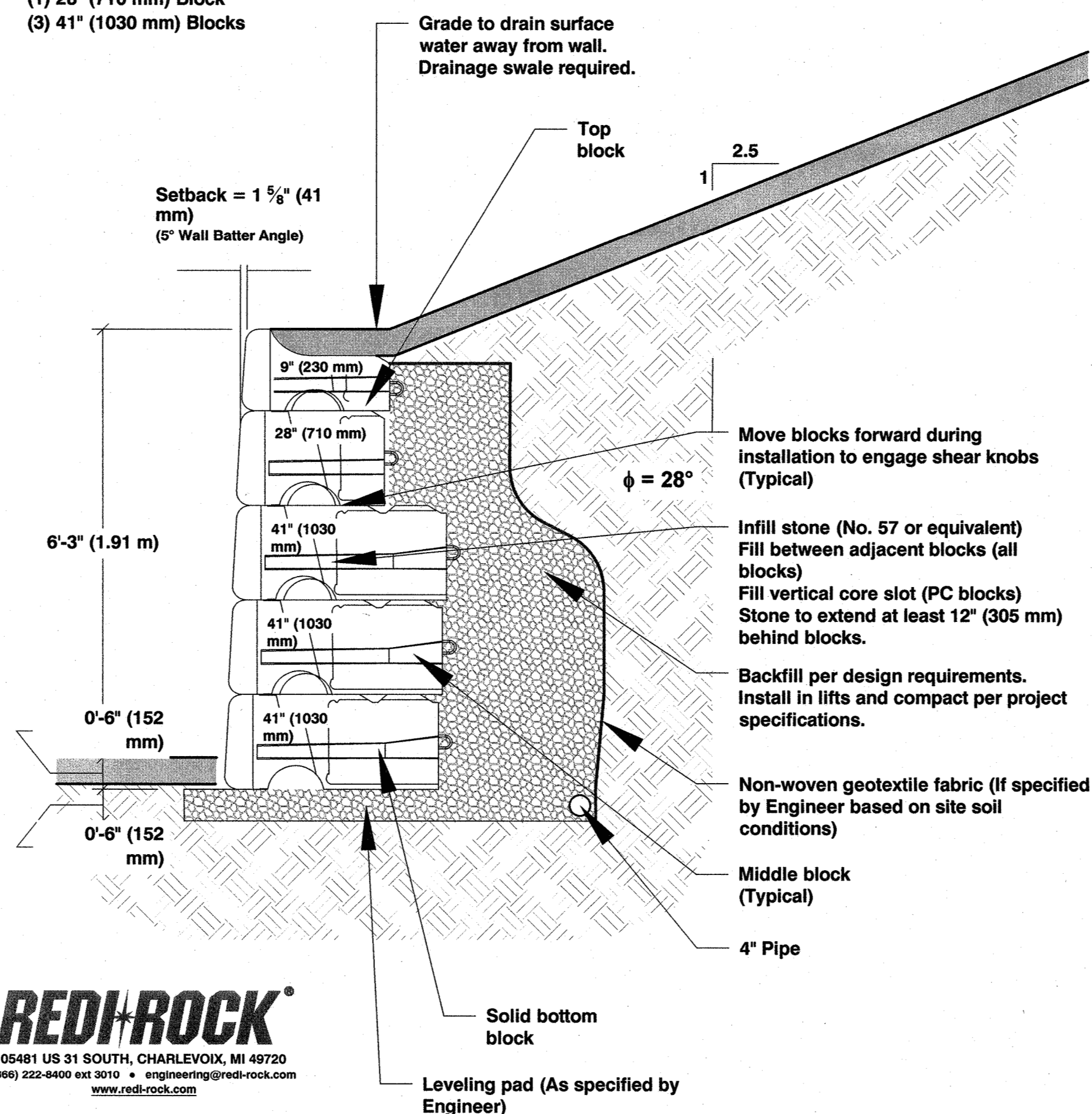
REDI ROCK WALL: 5 BLOCK SECTION
