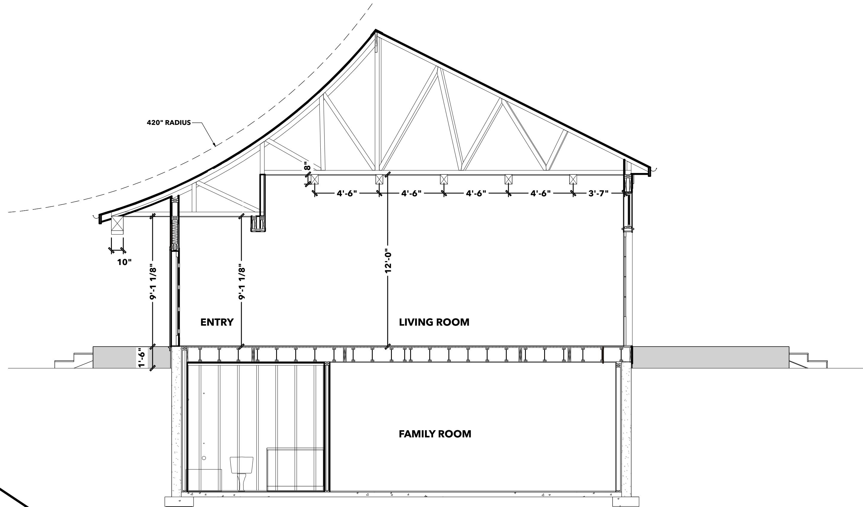
S11 CROSS SECTION 11 1/4 IN = 1 FT
