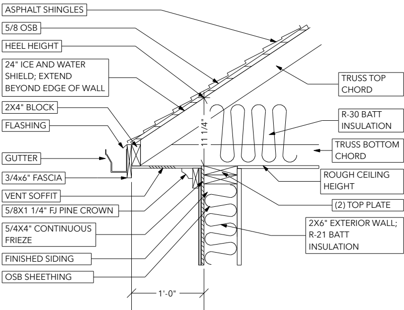
G 8:12 EAVE DETAIL SOFFITED
