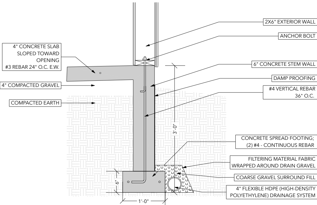
D GARAGE PERIMETER
