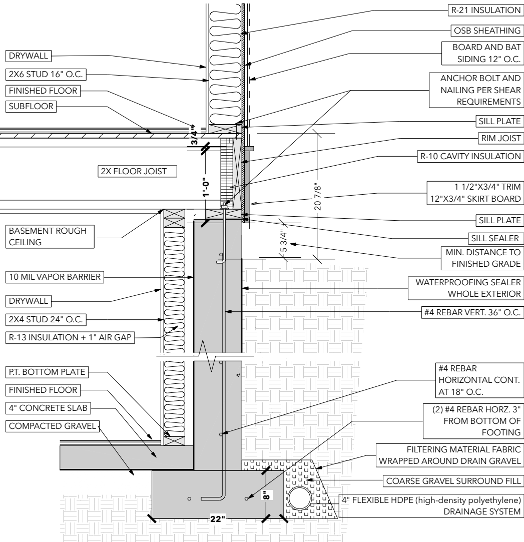
A FOUNDATION BASEMENT
