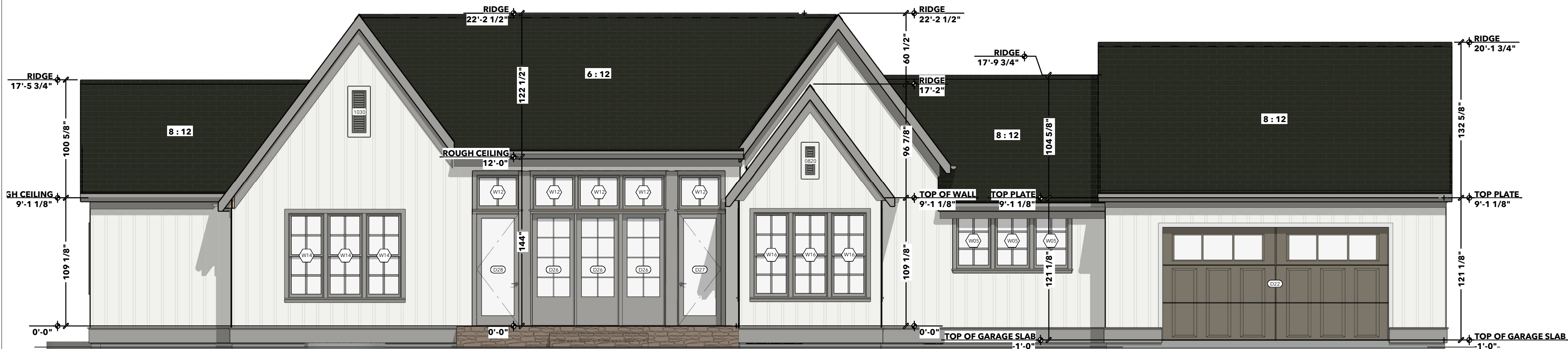
E3 EXTERIOR ELEVATION BACK 3/16 IN = 1 FT
