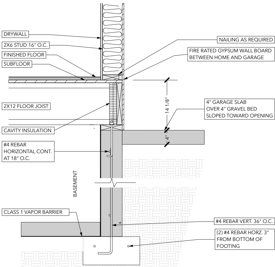
C GARAGE SLAB AT HOME TYP. FLOOR FOUNDATION
