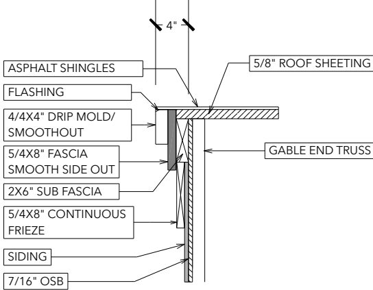
H GABLE END DETAIL SHORT
