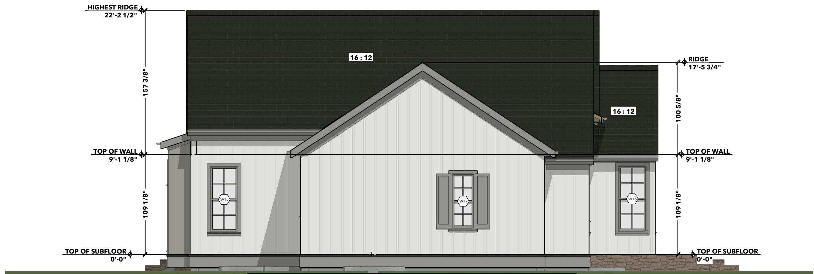
E4 EXTERIOR ELEVATION RIGHT 3/16 IN = 1 FT
