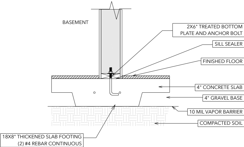
B INTERIOR FOOTING AT WALL
