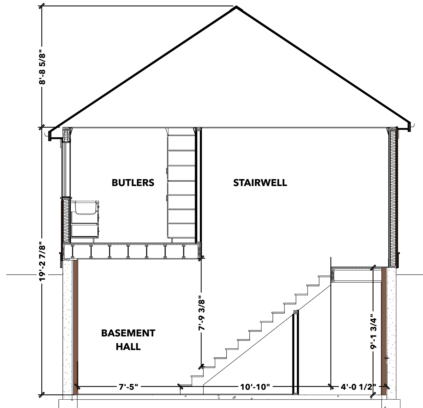
S12 CROSS SECTION 12 1/4 IN = 1 FT
