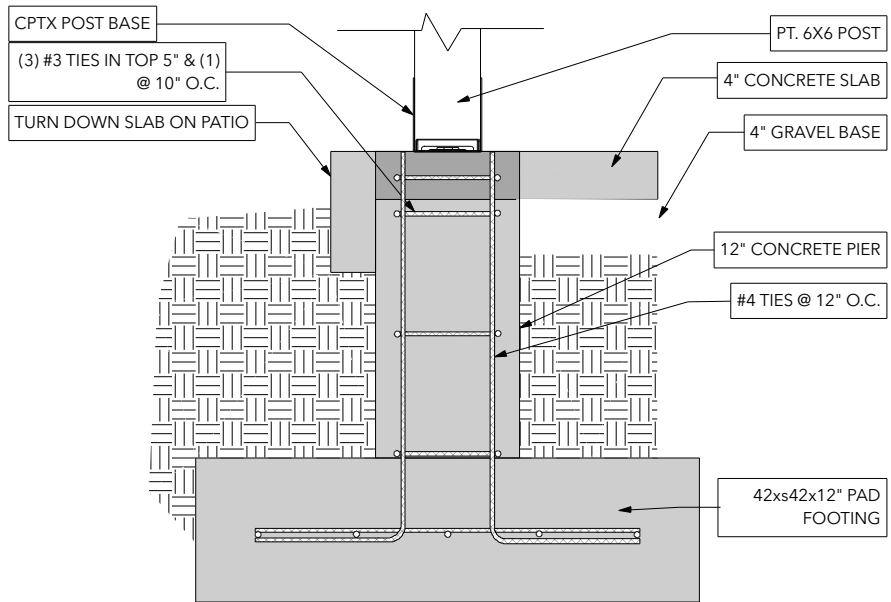
F COLUMN BASE
